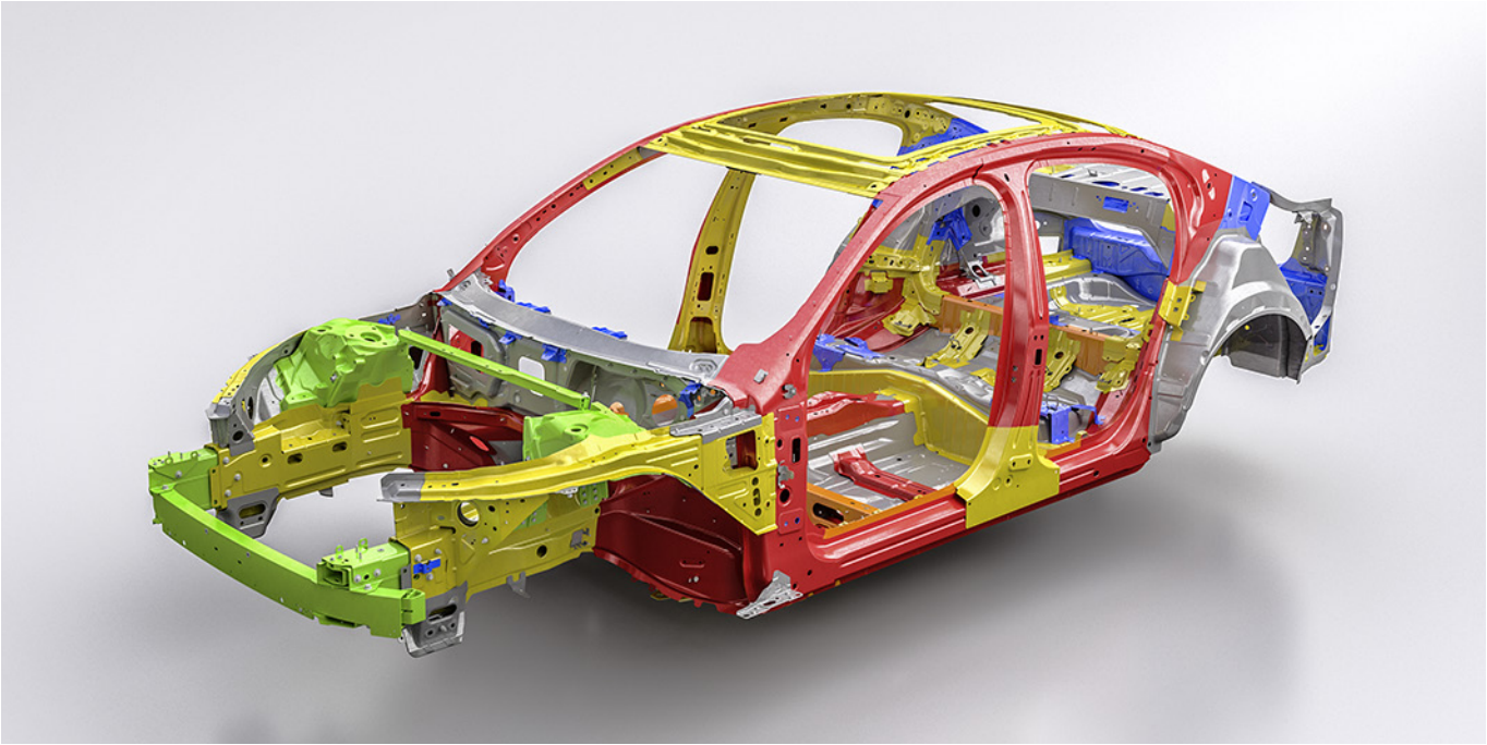
Volvo safety cage. The passenger compartment uses a high percentage of ultra high-strength boron steel to create a protective cage around everyone inside the car, while front and rear deformation zones help dissipate the crash energy. The safety belts and airbags work together to cushion you and your passengers in a controlled fashion.
